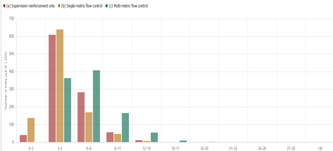
Figure 2: For each of 1,000 parameter draws, the year in which V \times L first exceeds C_{max} is recorded for each strategy. The rightmost bin, >30, indicates trials where no exceedance occurred within the 30-year simulation horizon. Supervision reinforcement alone, strategy (a), clusters in the early years. Single-metric flow control, strategy (b), delays exceedance moderately. Multi-metric flow control, strategy (c), pushes the majority of trials beyond the simulation horizon.
